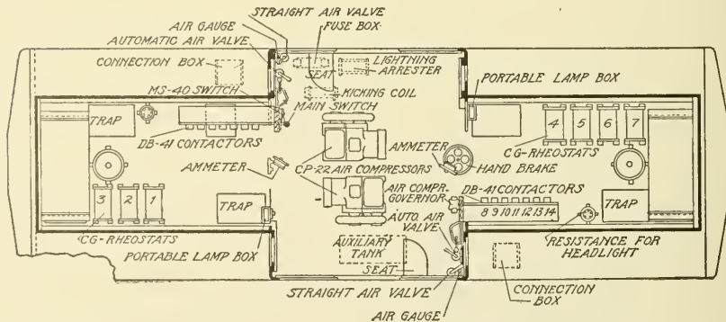
Fig. 244. Sectional Elevation and Plan of Typical Electric Locomotive
